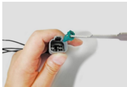
2.用力拉动取卸工具，把压板取出。 Pull the extraction tool until wedge is out of receptacle .
